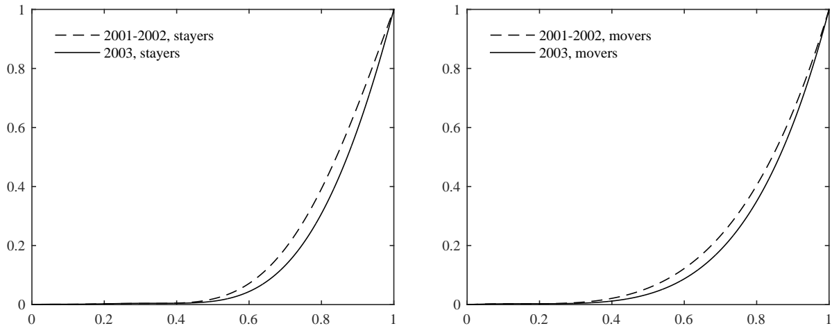
Figure 3: Sieve MLE estimates of F_{Y|X,S} .
